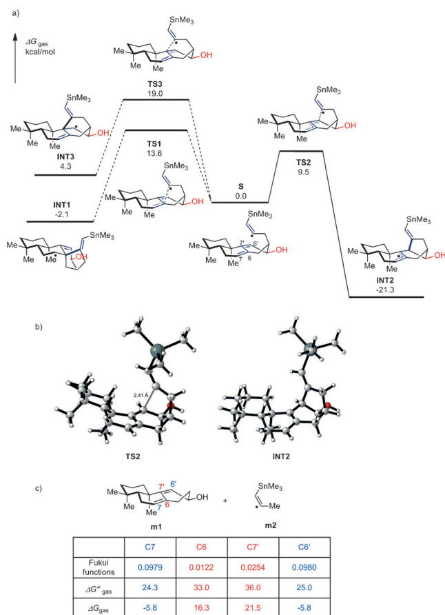
Figure 2. a) Computed free-energy profile of dienyne reductive radical cyclization of 5 at the UB3LYP/SDD-6-311 + G(d,p)//UB3LYP/SDD-6-31G(d) level of theory. b) Computed structures of TS2 and INT2 . c) Computed Fukui functions at C7, C6, C7', and C6' of the model substrate of m1 , and the activation free energies and reaction free energies for the corresponding radical additions of m2 to m1 at these positions, calculated at the (U)B3LYP/SDD-6-31G(d) level of theory. Energies in \text{kcal mol}^{-1} .
